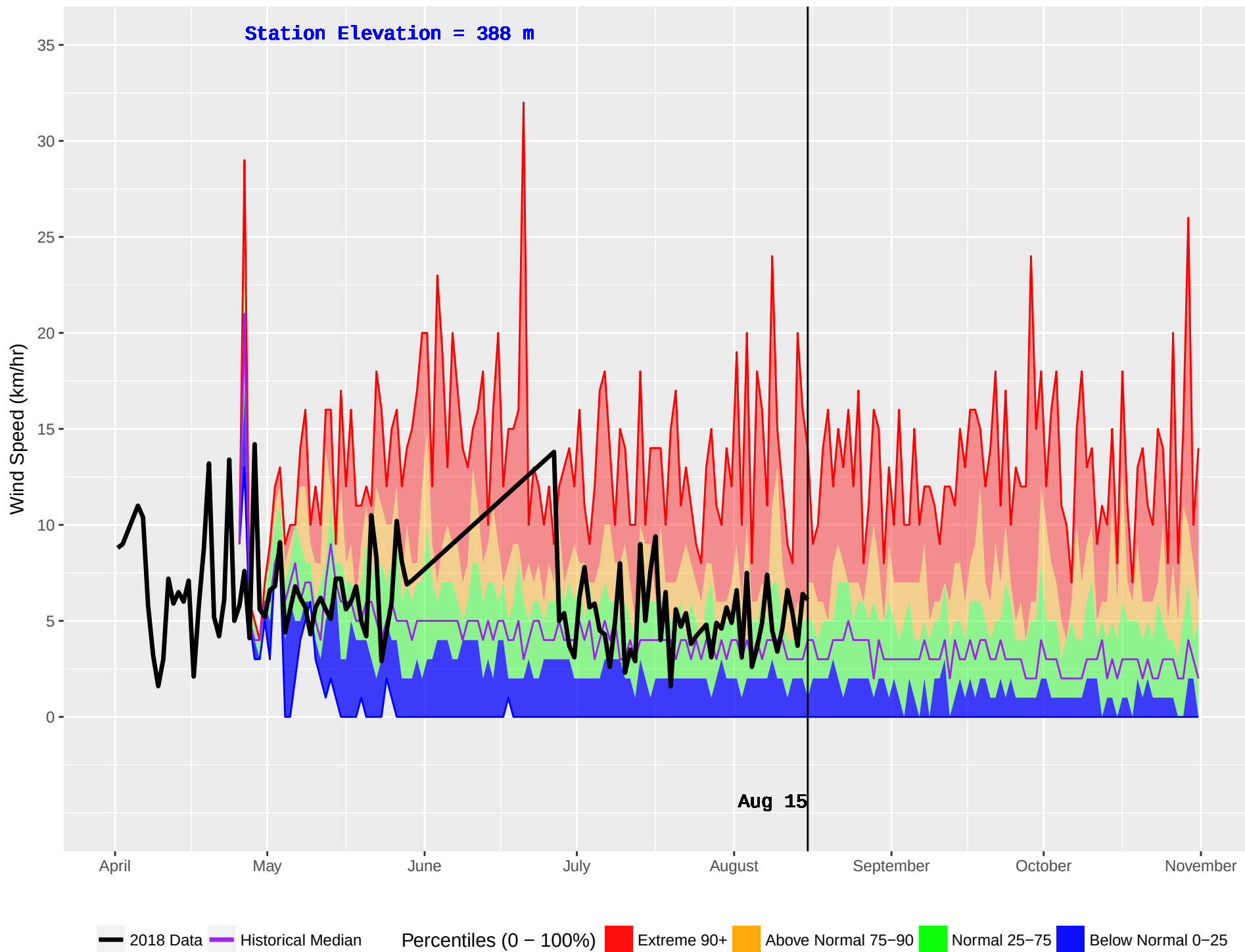
BELL-IRVING (432) : Historical (1986–2016) and Current (2018) Daily Wind Speed
