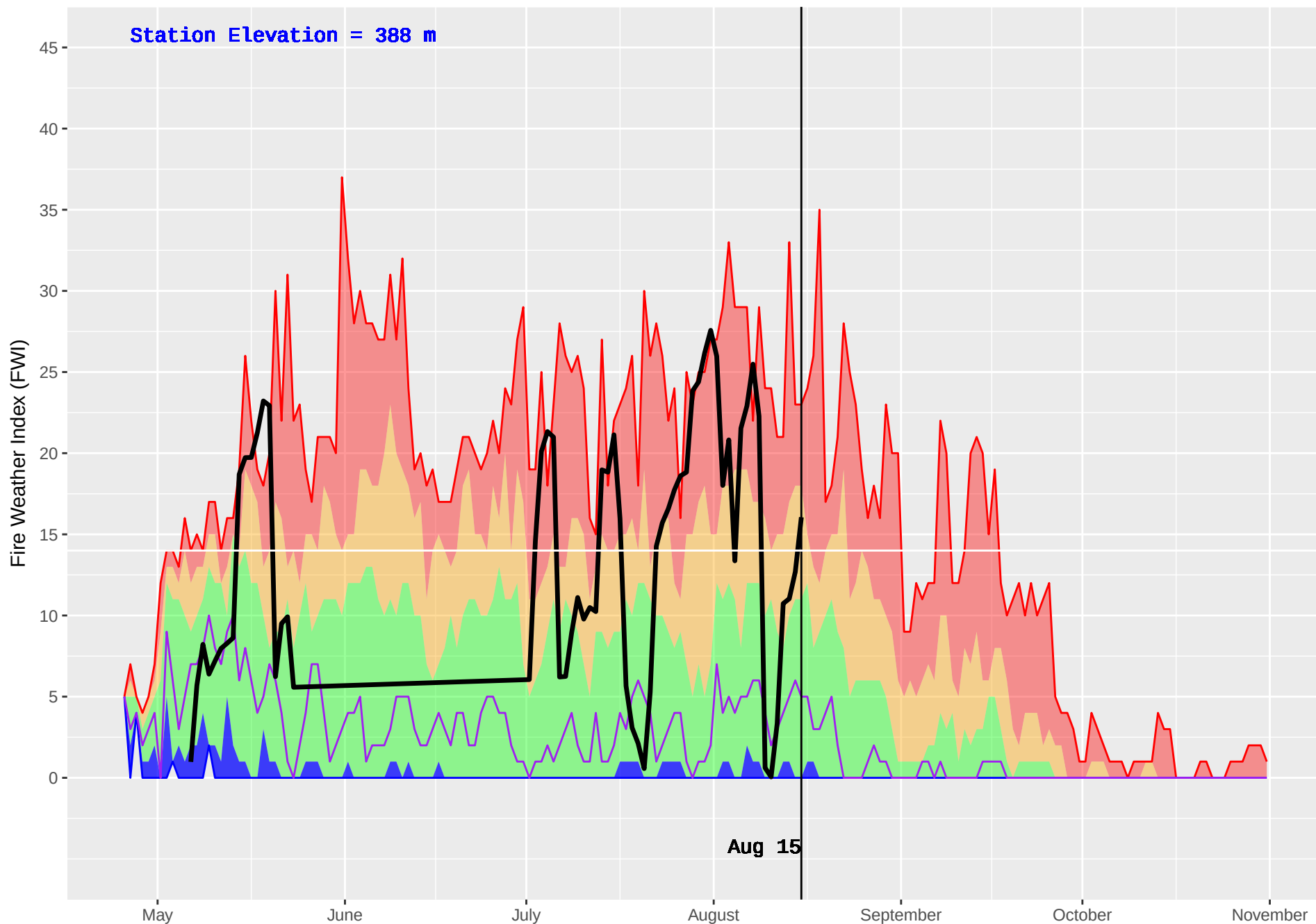
BELL-IRVING (432) : Historical (1986–2016) and Current (2018) Daily Fire Weather Index (FWI)
