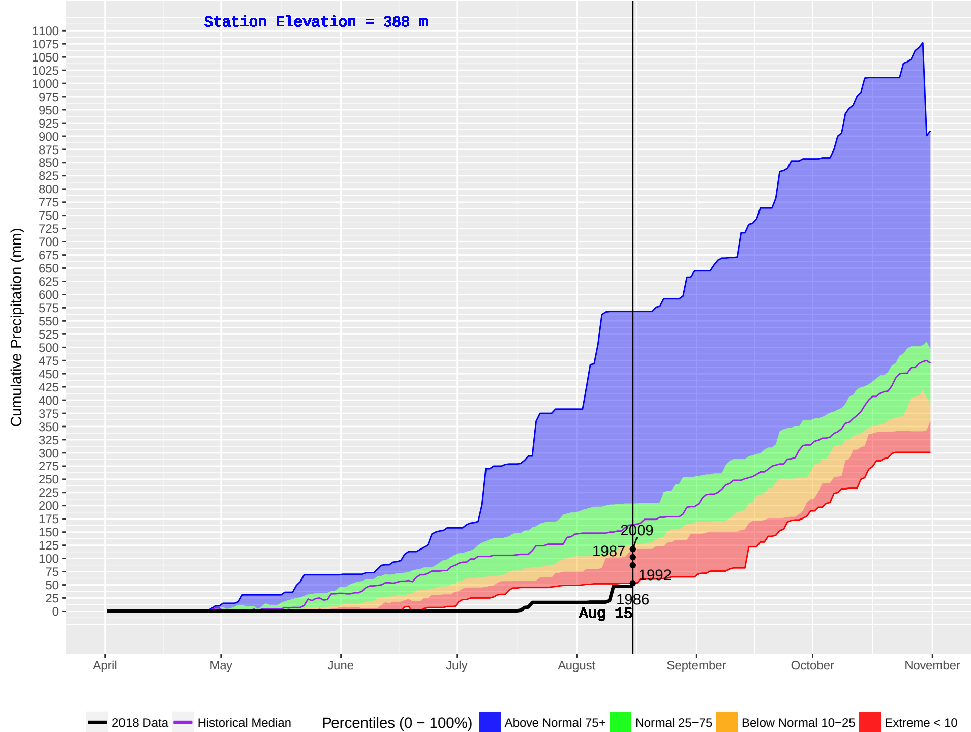
BELL-IRVING (432) : Historical (1986–2016) and Current (2018) Daily Cumulative Precipitation
