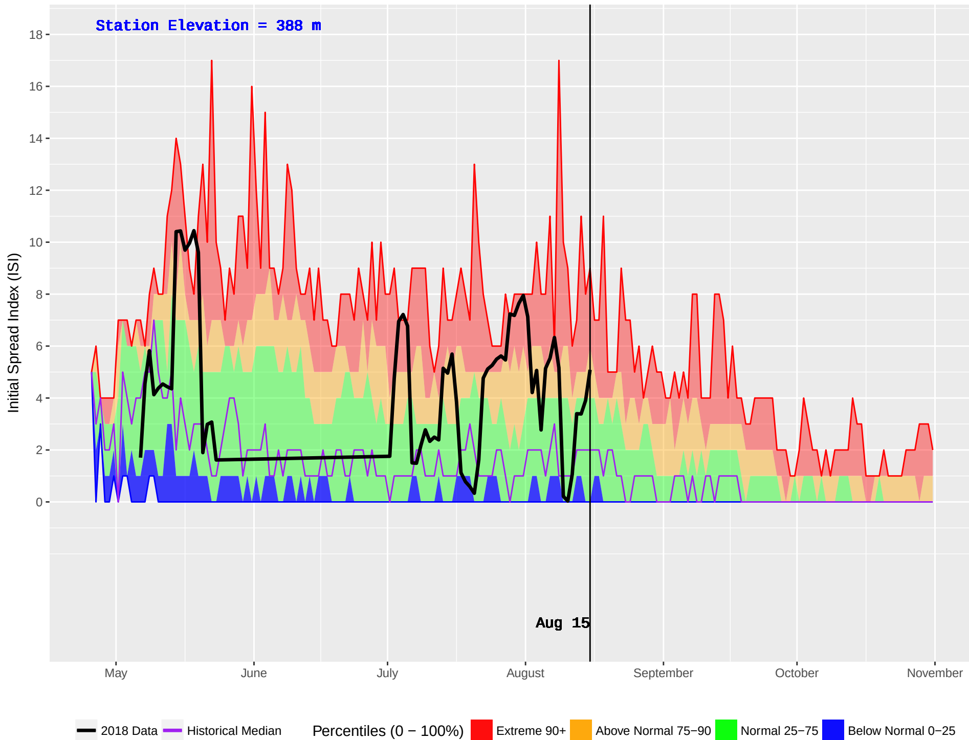
BELL-IRVING (432) : Historical (1986–2016) and Current (2018) Daily Initial Spread Index (ISI)
