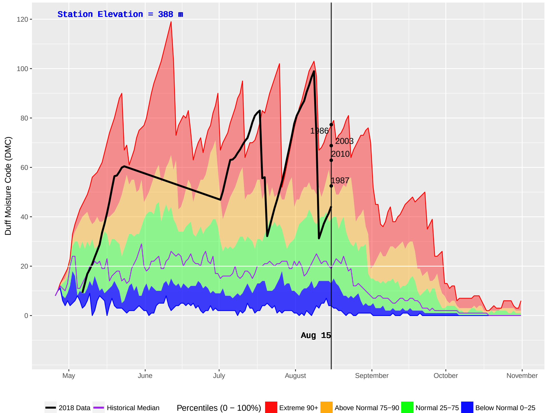
BELL-IRVING (432) : Historical (1986–2016) and Current (2018) Daily Duff Moisture Code (DMC)
