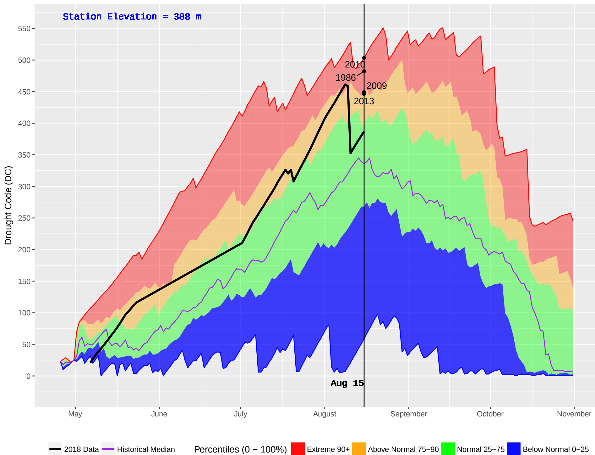
BELL-IRVING (432) : Historical (1986–2016) and Current (2018) Daily Drought Code (DC)
