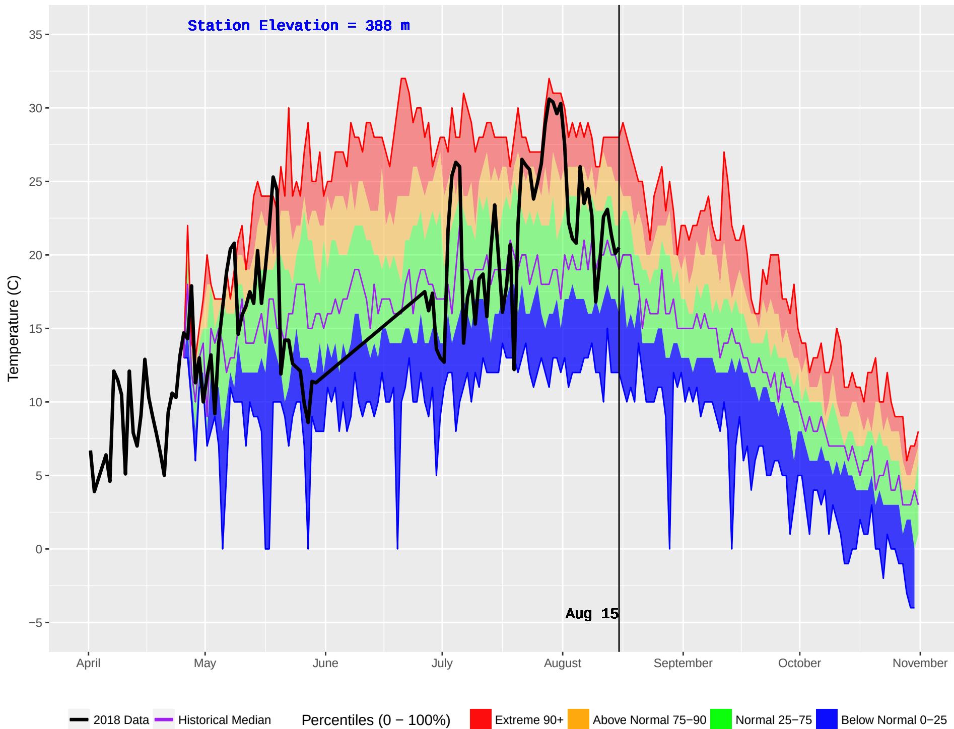
BELL-IRVING (432) : Historical (1986–2016) and Current (2018) Daily Temperature
