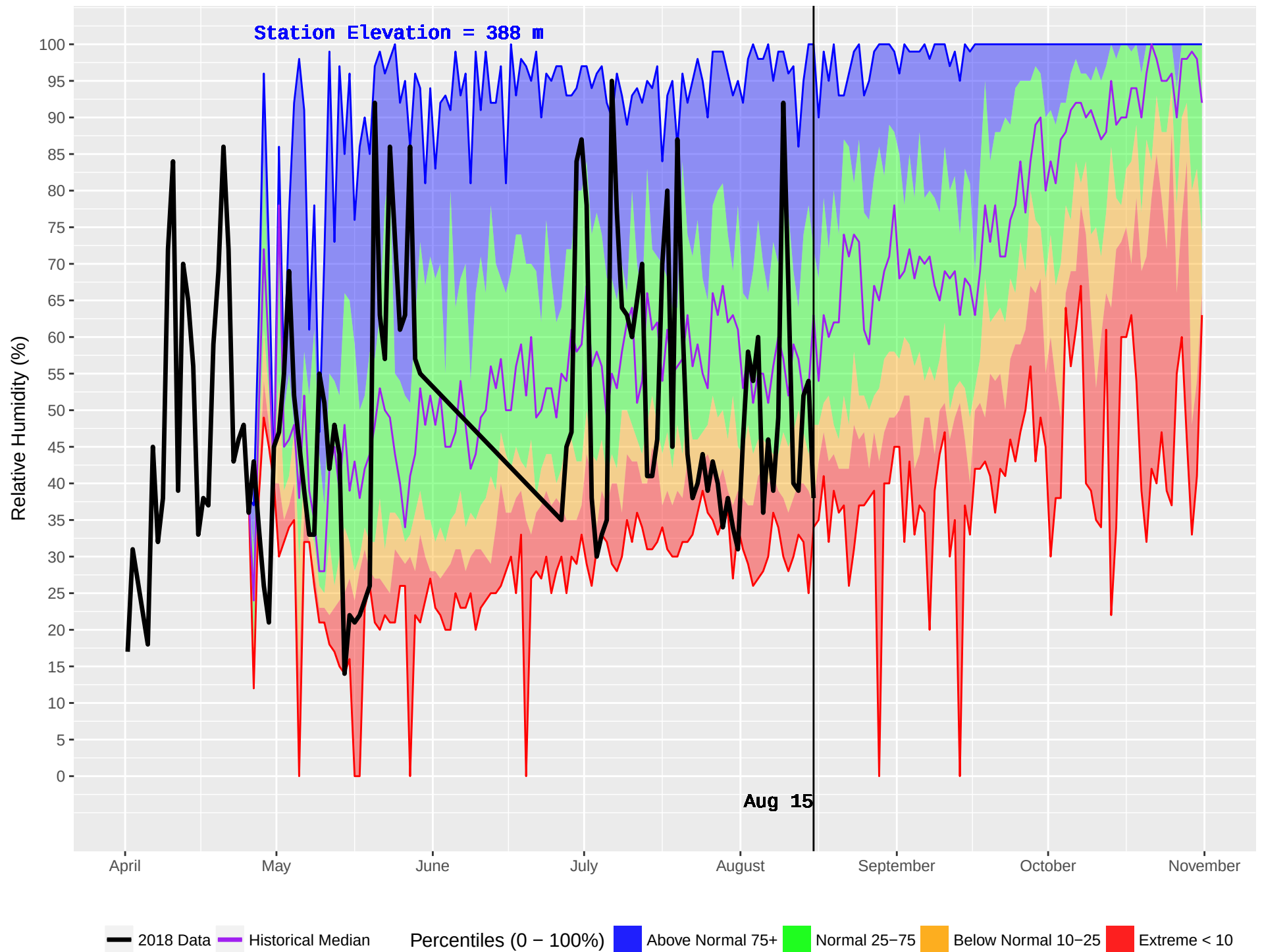
BELL-IRVING (432) : Historical (1986–2016) and Current (2018) Daily Relative Humidity
