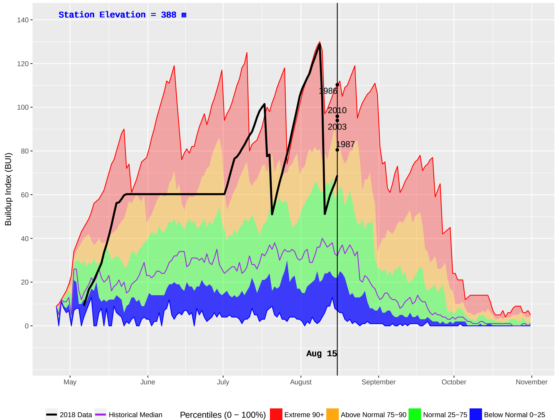
BELL-IRVING (432) : Historical (1986–2016) and Current (2018) Daily Buildup Index (BUI)
